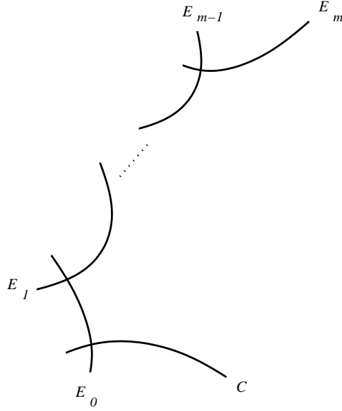
FIGURE 1. The chain of exceptional curves in \tilde{\mathcal{Y}} .
